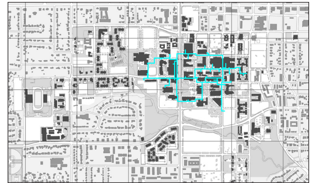
UT Arlington Chilled Water System
